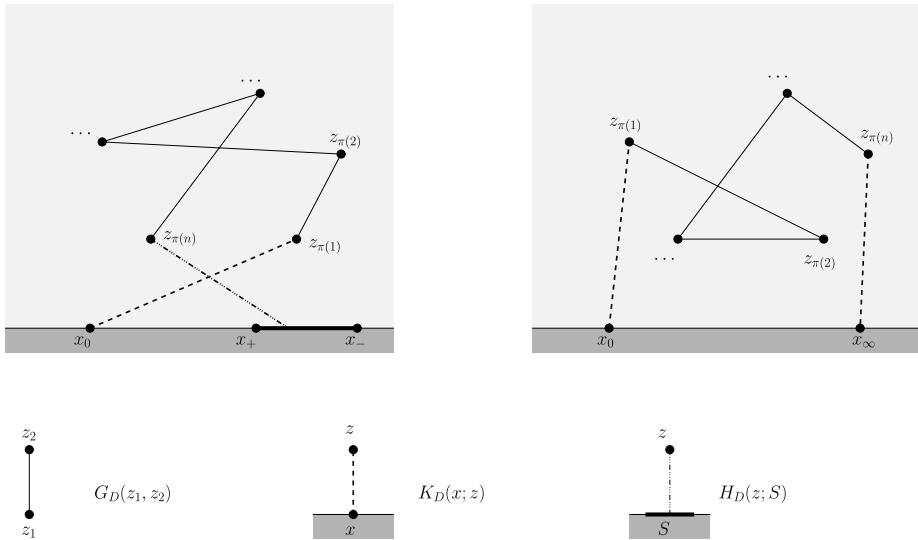
Fig. 1 Example diagrams representing the terms in the local time multipoint correlation functions. Dipolar case (15) is on the left and chordal case (16) on the right
