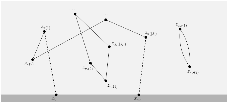
Fig. 2 Example diagram for a term appearing in the correlation function (20) of fields :\chi^-\chi^+:\mathbb{H} . The component containing boundary points x_0 and x_\infty corresponds to J whereas the rest of the connected components correspond to J_1, \dots, J_s . Within each component J_r we sum over inequivalent cyclic orderings \pi_r of it
